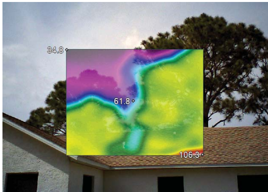
This is the same house, at the same moment through a high resolution infrared lens. The blue lines show cold air pouring out of a roof vent. The result of a defective range hood installation.
